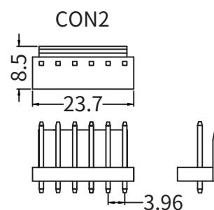
CON2
