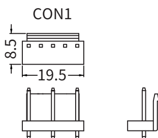
CON1
